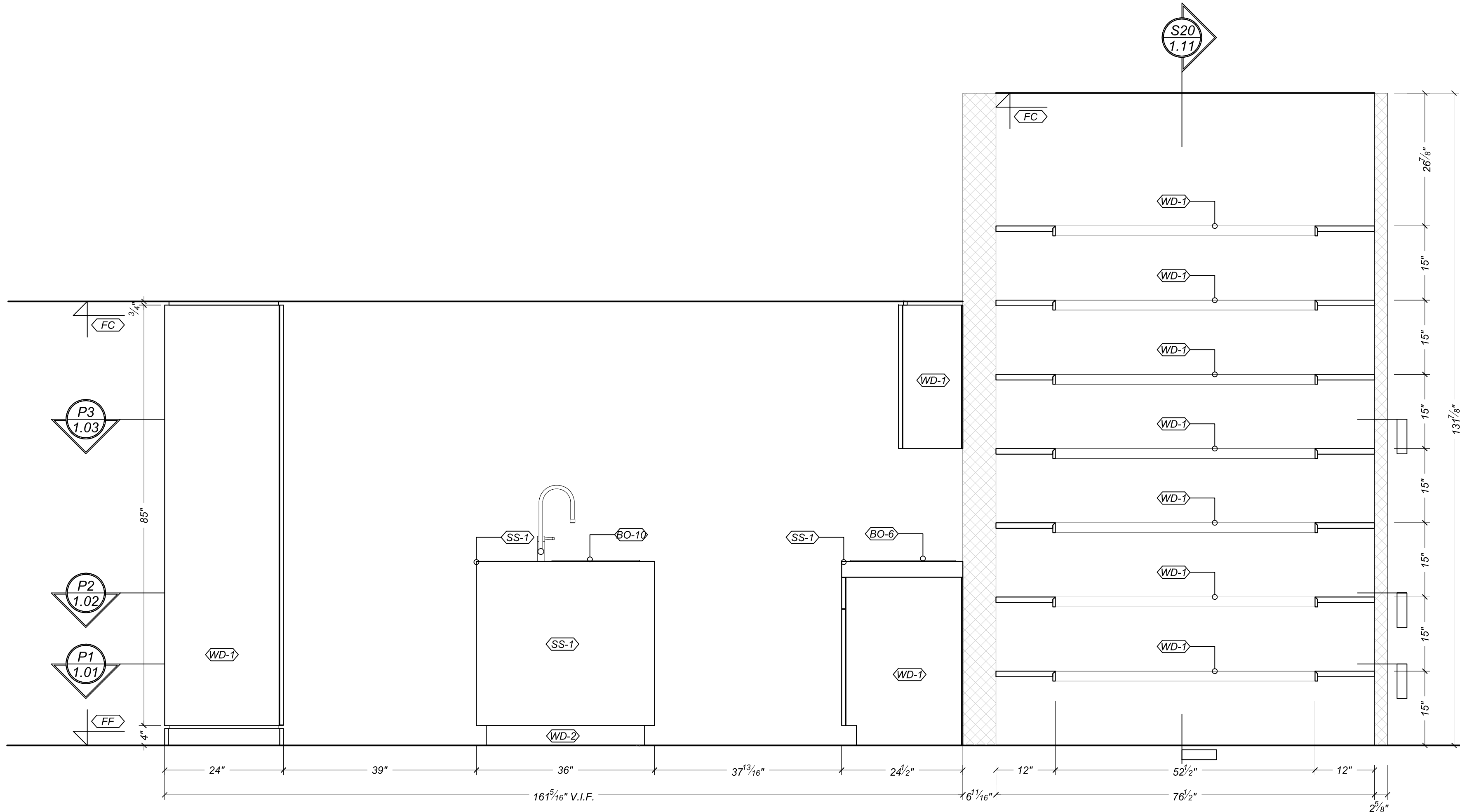
FRONT/SIDE ELEVATION @ KITCHEN & PANTRY SCALE: 3/4"=1'-0"
