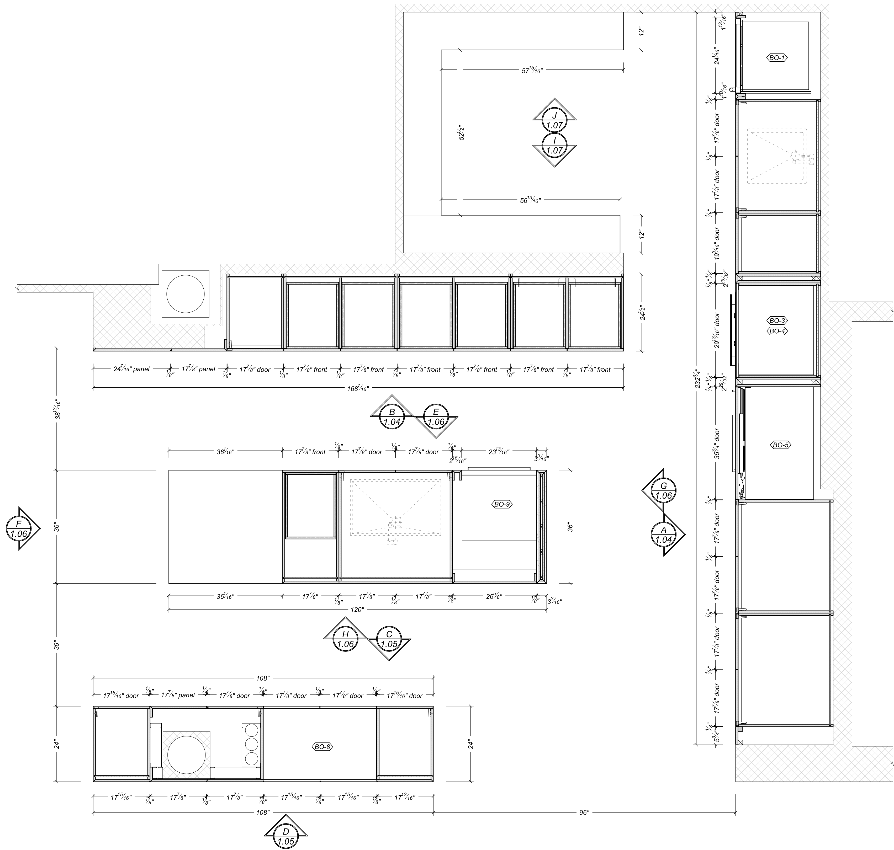
SECTION P2 PLAN @ KITCHEN & PANTRY SCALE: 3/4"=1'-0"
