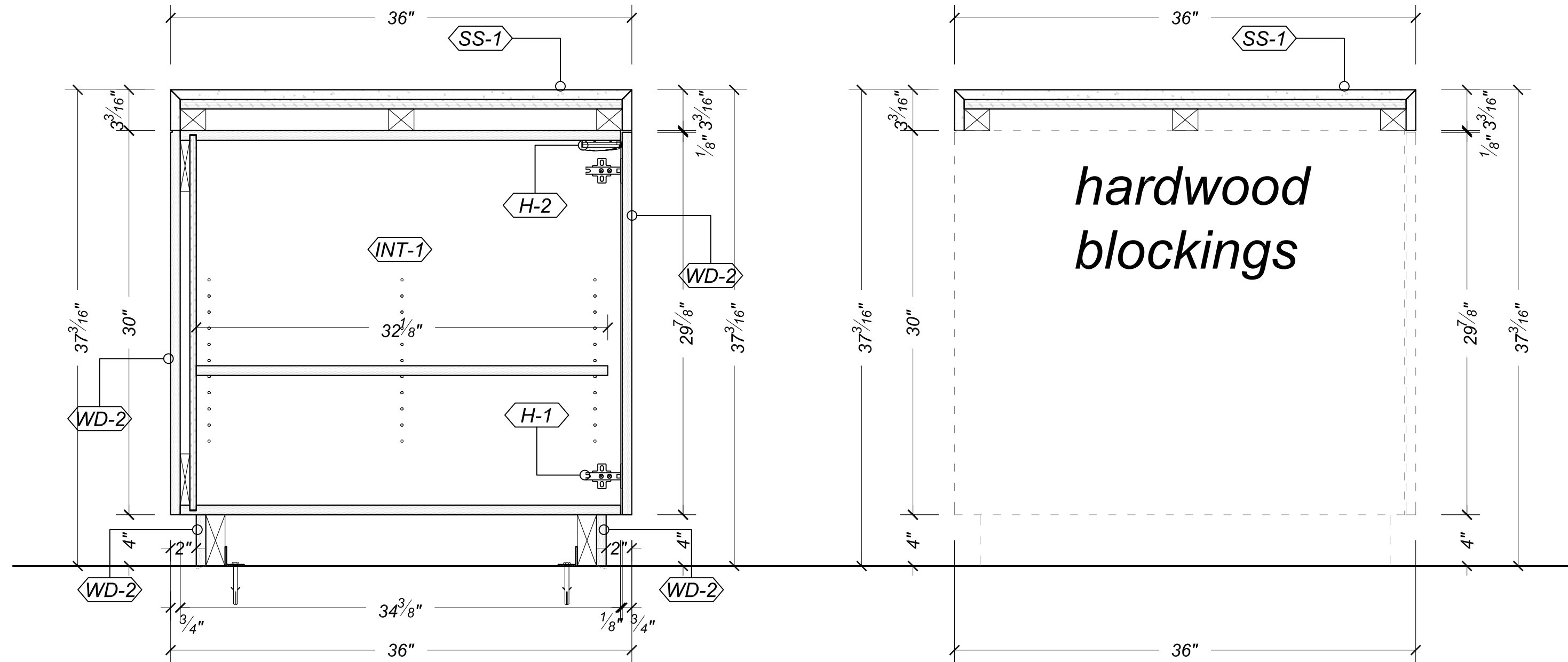
VERTICAL S18 SECTION @ ISLAND SCALE: 1-1/2"=1'-0"
