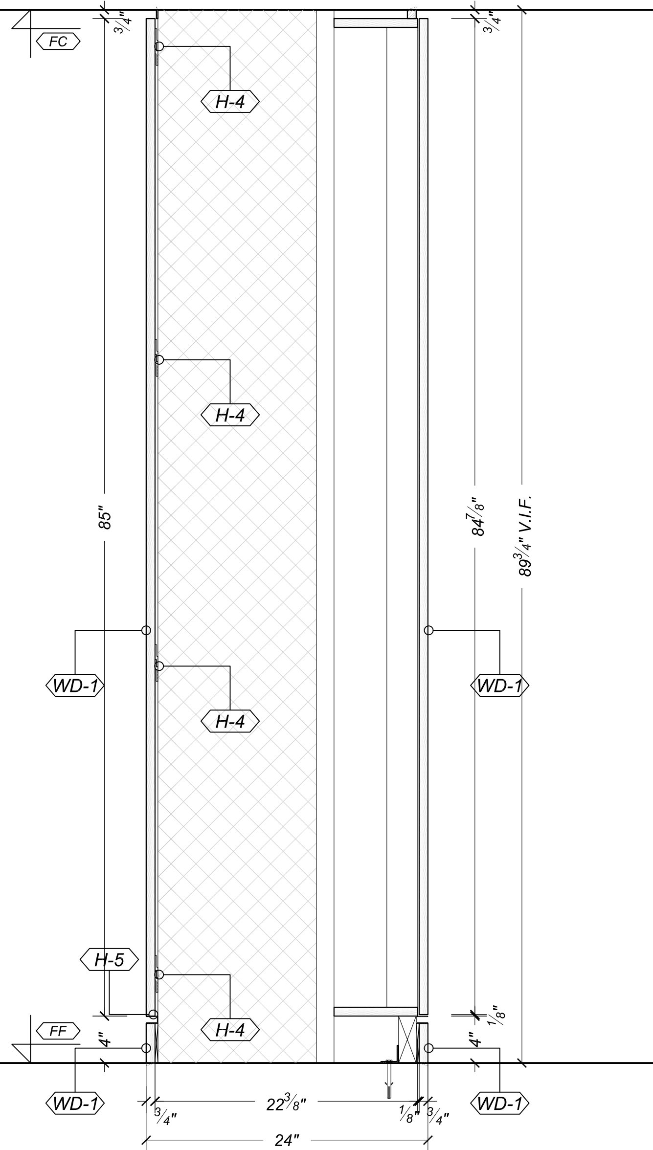
VERTICAL S15 SECTION @ KITCHEN SCALE: 1-1/2"=1'-0"
