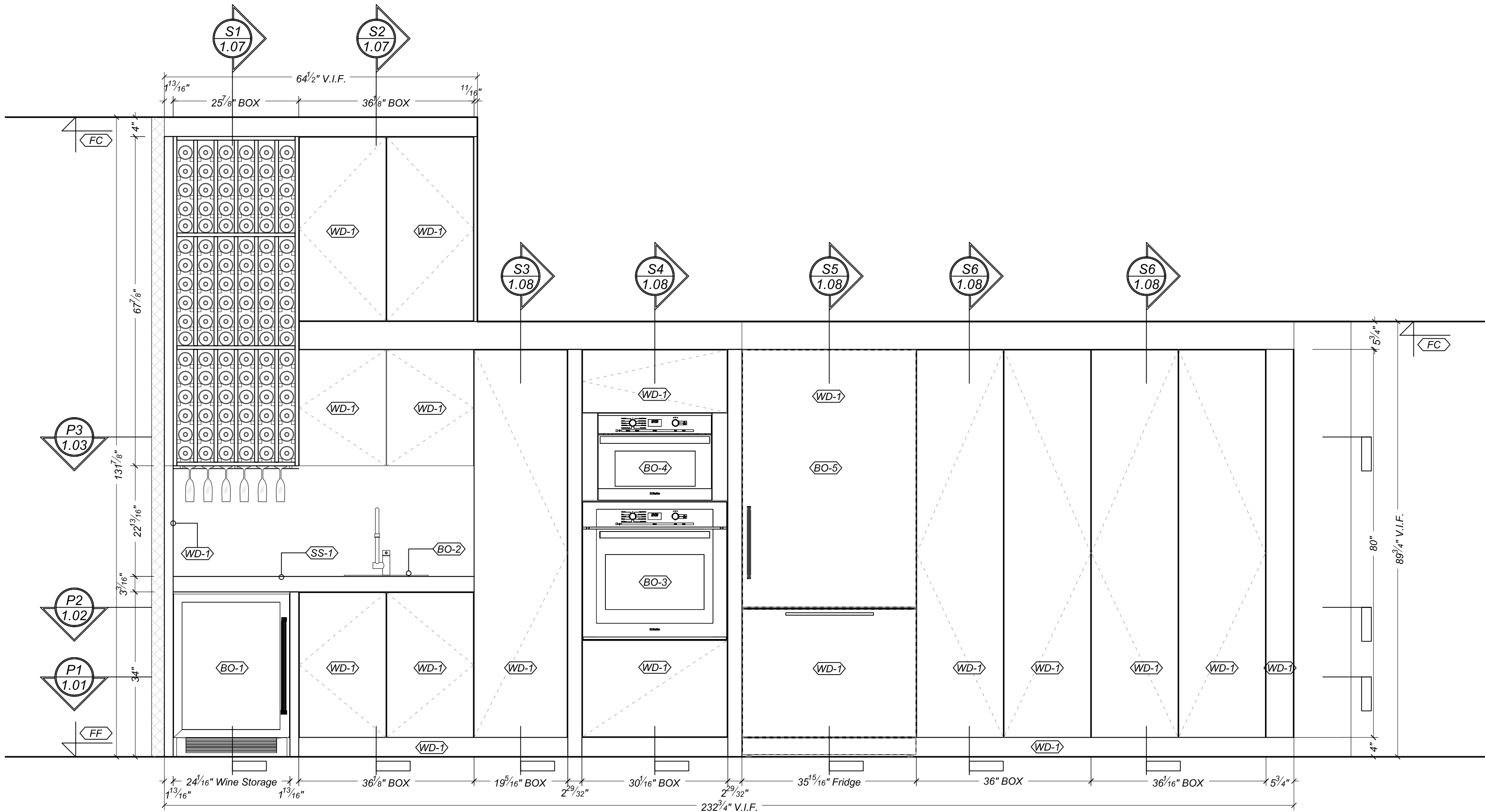
FRONT ELEVATION @ KITCHEN & PANTRY SCALE: 3/4"=1'-0"
