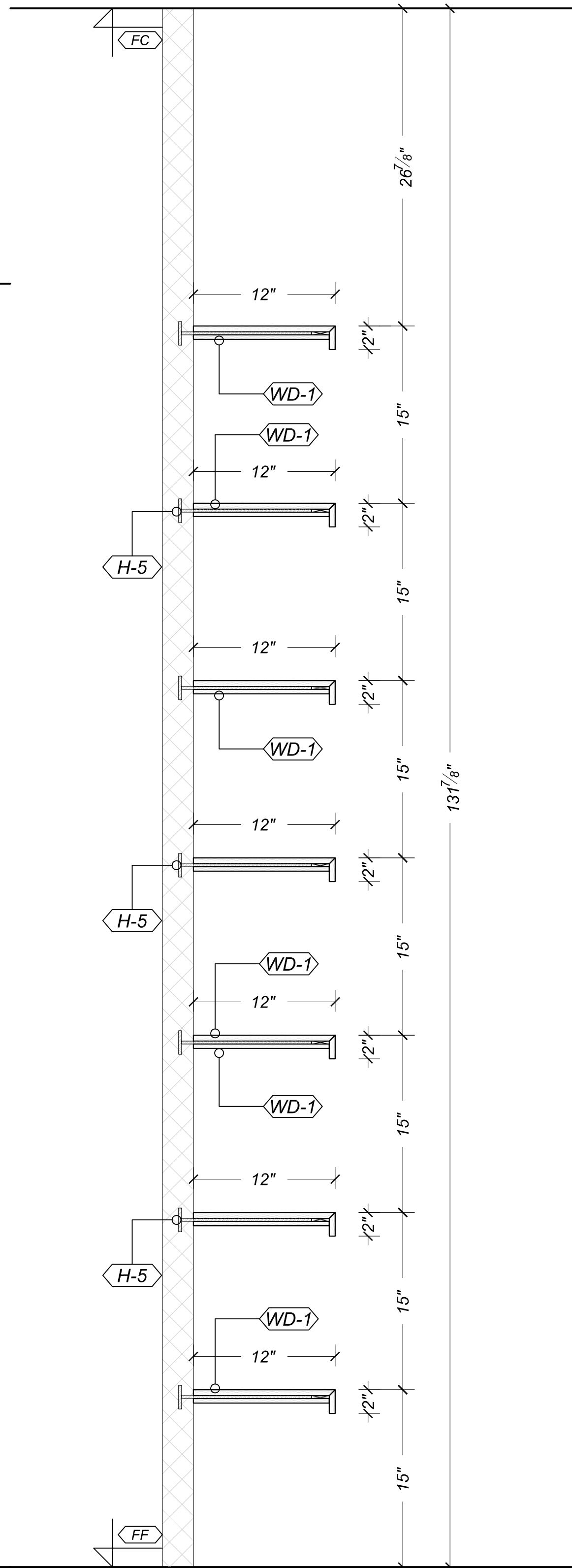
VERTICAL S20 SECTION @ PANTRY SCALE: 1-1/2"=1'-0"
