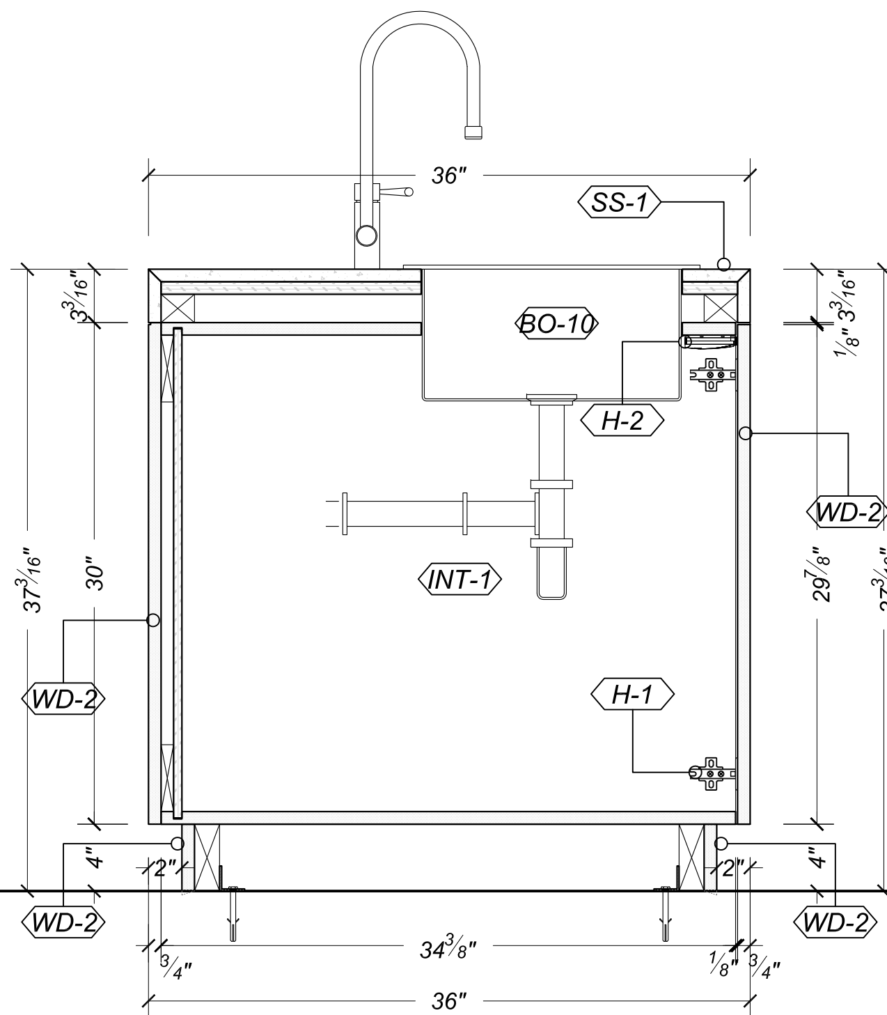
VERTICAL S17 SECTION @ ISLAND SCALE: 1-1/2"=1'-0"
