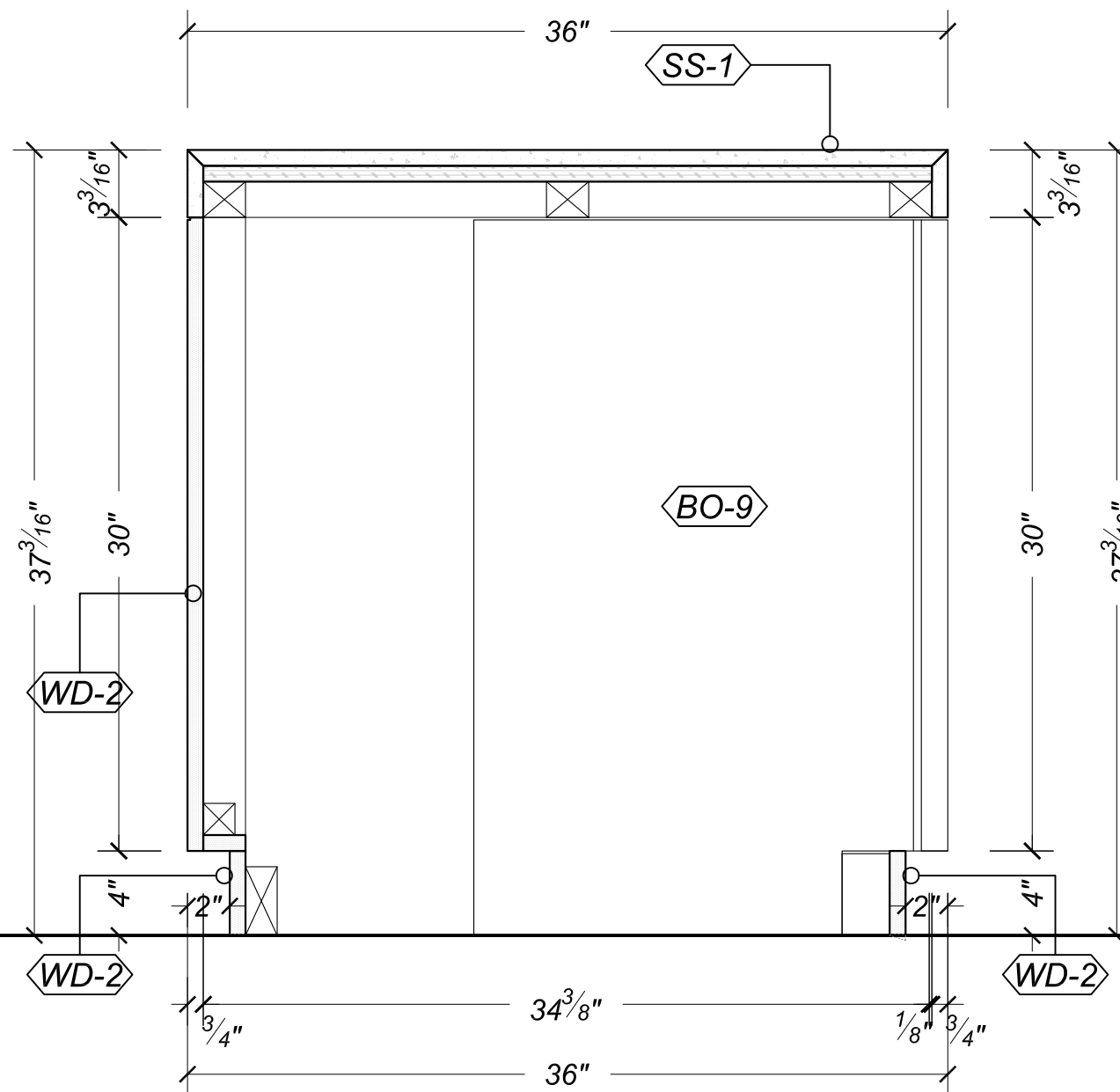
VERTICAL S16 SECTION @ ISLAND SCALE: 1-1/2"=1'-0"
