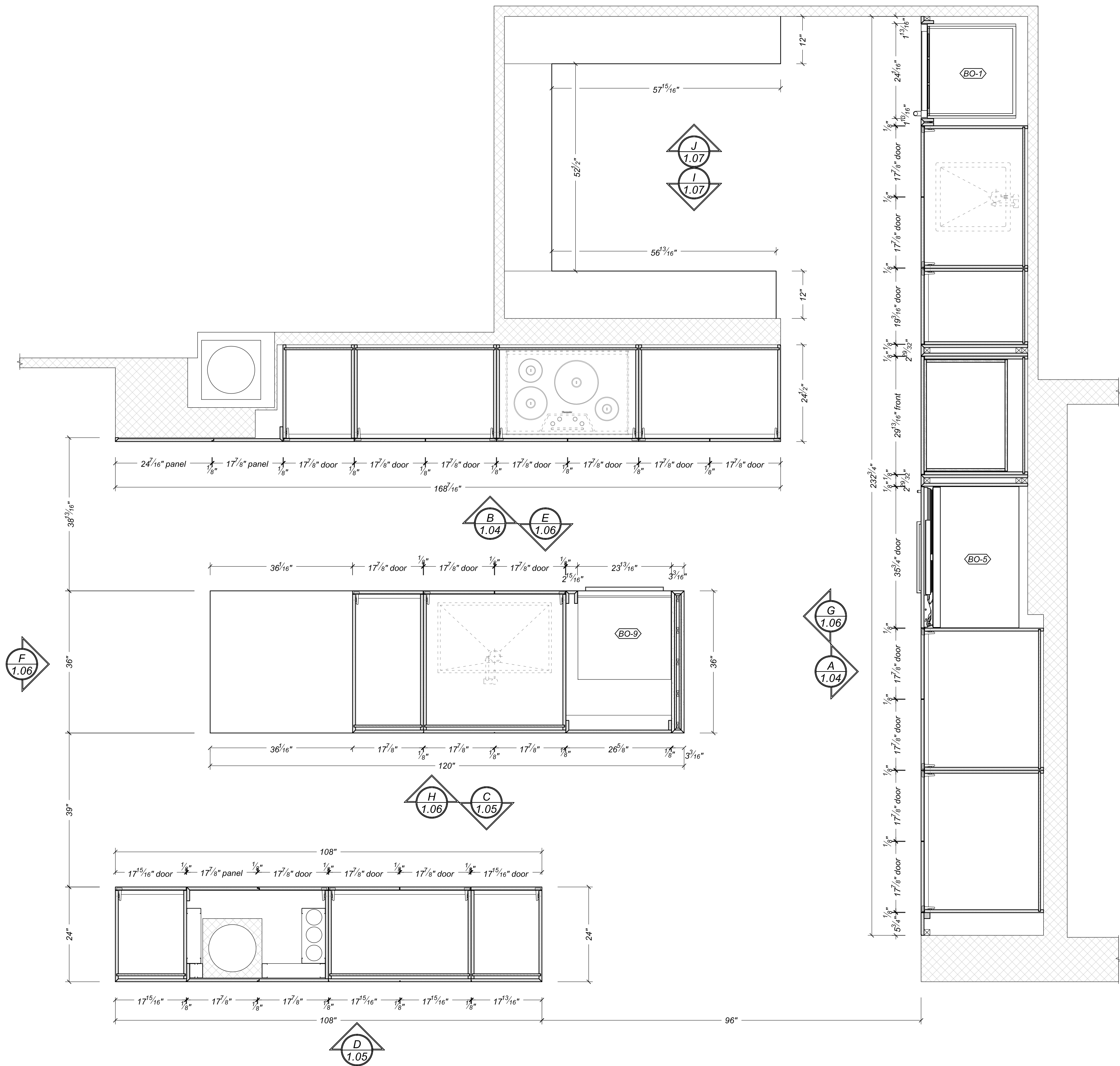
SECTION P1 PLAN @ KITCHEN & PANTRY SCALE: 3/4"=1'-0"
