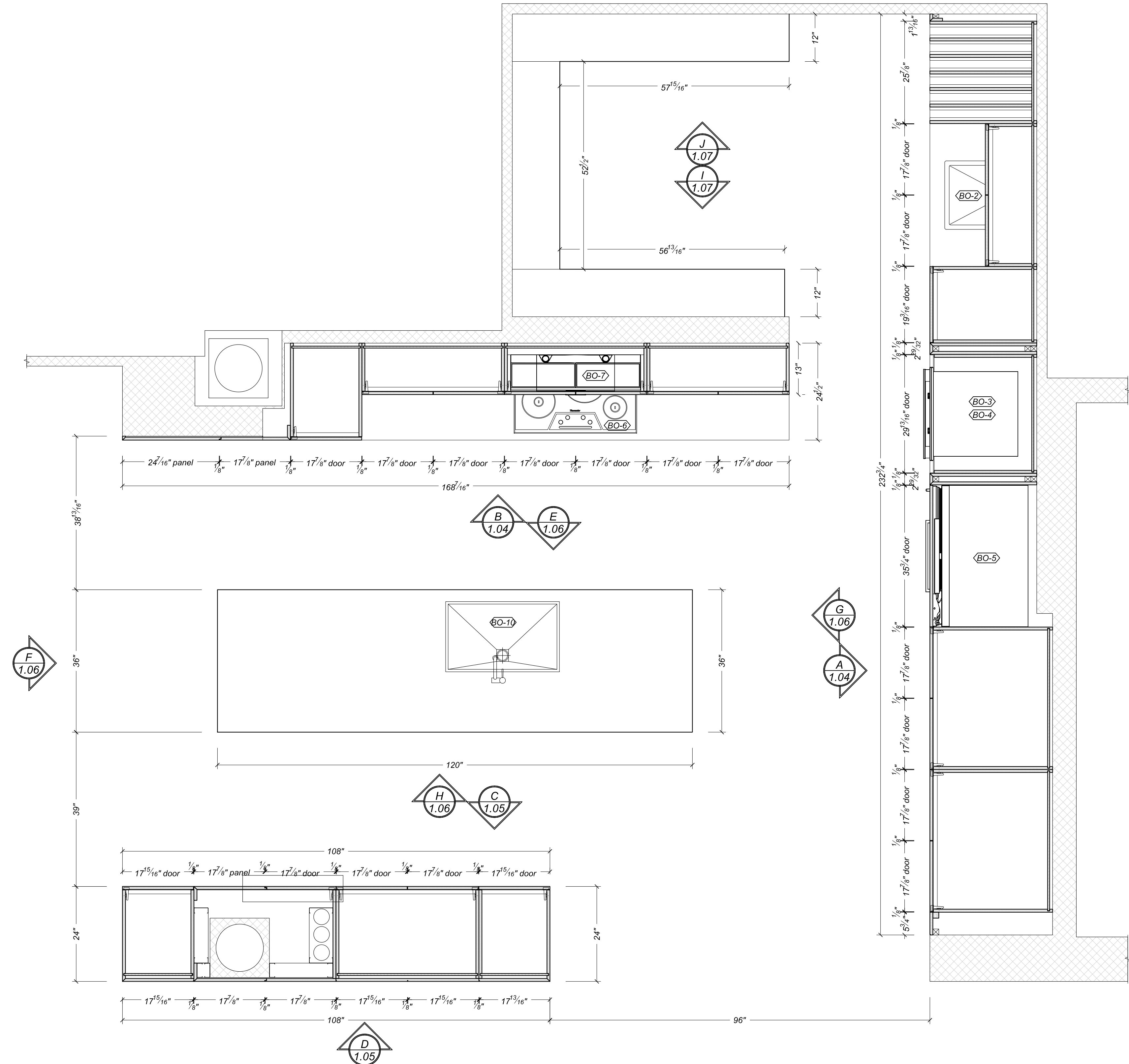
SECTION P3 PLAN @ KITCHEN & PANTRY SCALE: 3/4"=1'-0"
