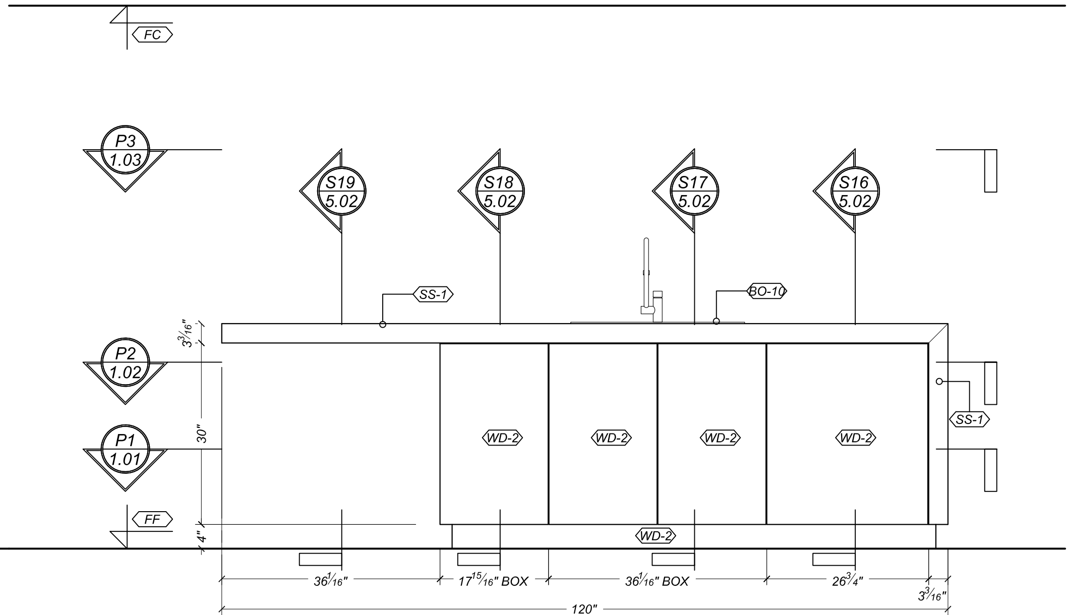
FRONT ELEVATION @ ISLAND SCALE: 3/4"=1'-0"
