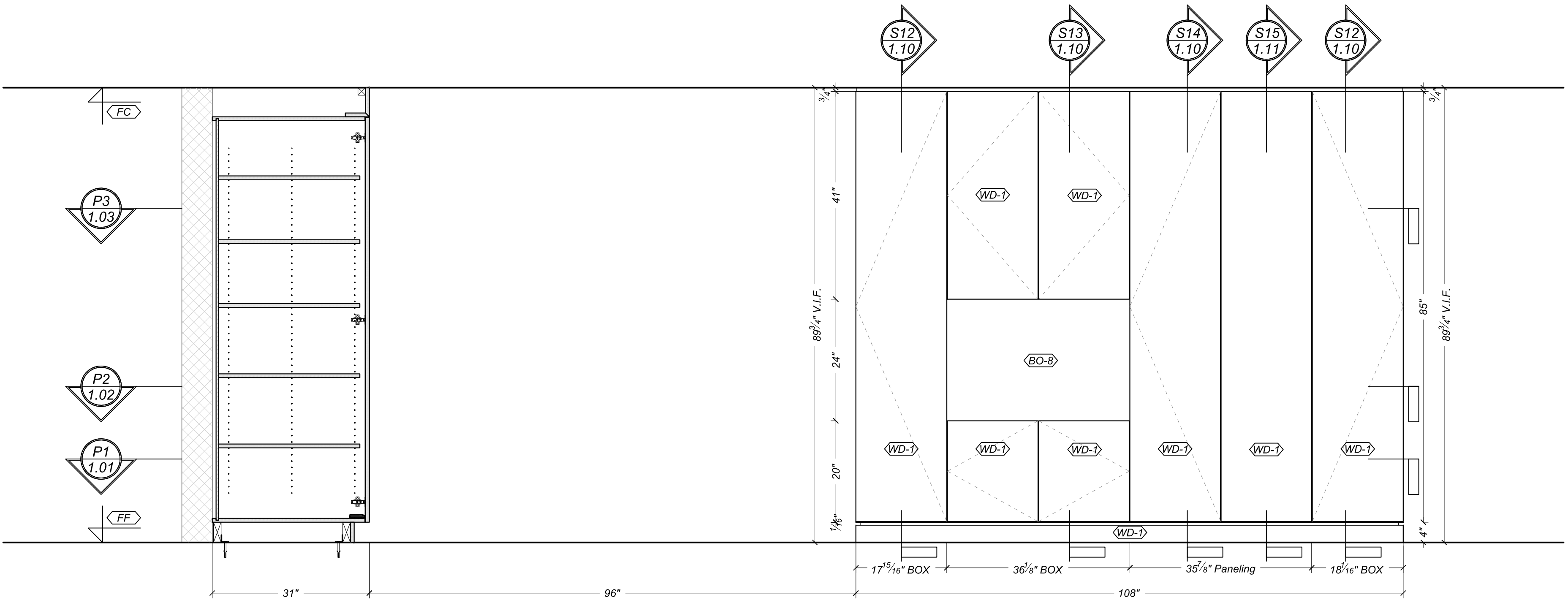
FRONT ELEVATION @ KITCHEN SCALE: 3/4"=1'-0"
